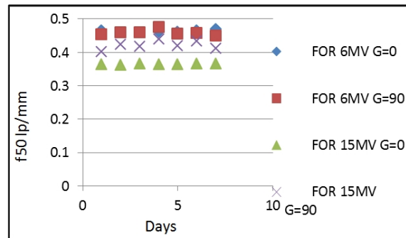
FIG. 6: Plot of f_{50} recorded on a daily basis for the as1000 portal imaging system with Gantry Angle 0^\circ and 90^\circ at 6MV and 15MV for days.
